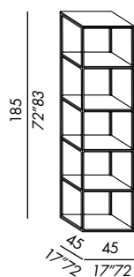
libreria / bookcase 45
