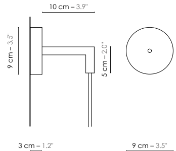
Wall plate
