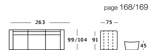
Composizione / Arrangement / Composition F + Art. 13
