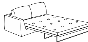
SIDE modules W 168- 188- 208 | H 82 | D 96 cm Mattress W 120-140-160 | D 175+15 | H 12 cm
