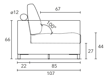
high back rest version
