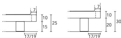
Standard feet for MEDIUM bed frame and upon request for MEDIUM 30 cm H bed frame.
