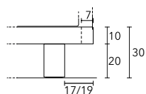
Standard feet for MEDIUM bed frame and upon request for MEDIUM 30 cm H bed frame.
