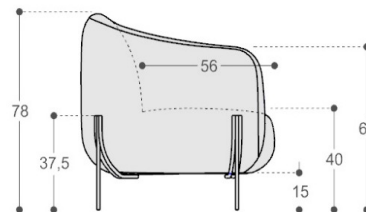
Vista laterale Side view
