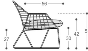
Vista laterale Side view
