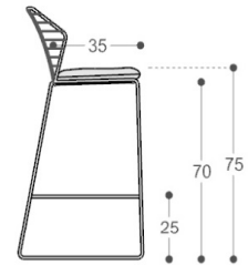
Vista laterale Side view
