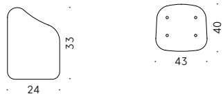
Seat cushion.
