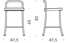
Stool.
