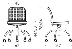
Swivel chair without armrests.
