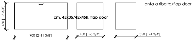
cm. 45x35/45x45h. open unit with black glass fumè
