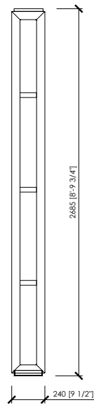
ceiling column
