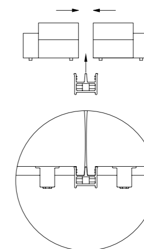
Stitching for element with armrest. The seat of the end element is curved on one side. When in composition, the element must be joined from the side shown by the arrow.
