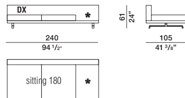
island element with tray (60x90) IV180A dx - sx
