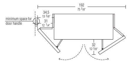
plan - measurements
