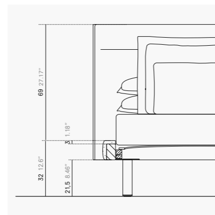
LEG6X6W Solid walnut. Noyer massif. Nogal macizo. 6 x 6 H21.5 2.36" x 2.36" H8.46"
