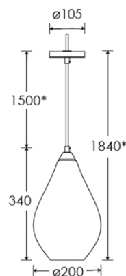
Dimensions in mm and approximate *Adjustable flex
