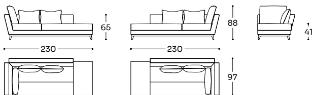
PFD - E08 / PFD - E09
