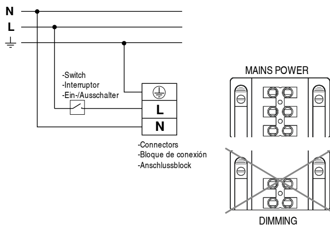
NO DIMMING Diagram Y
